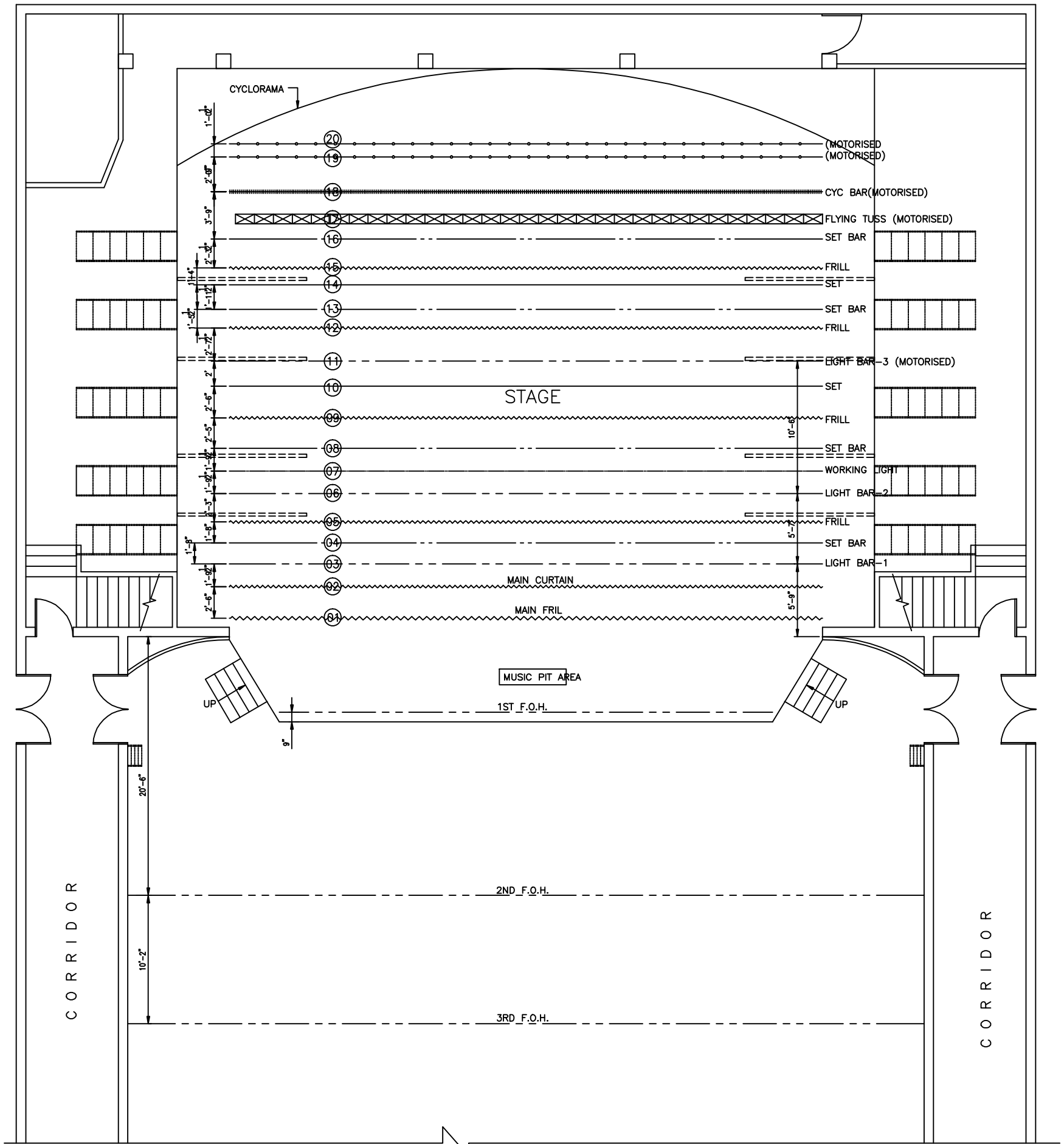
AUDITORIUM - STAGE BAR SYSTEM
