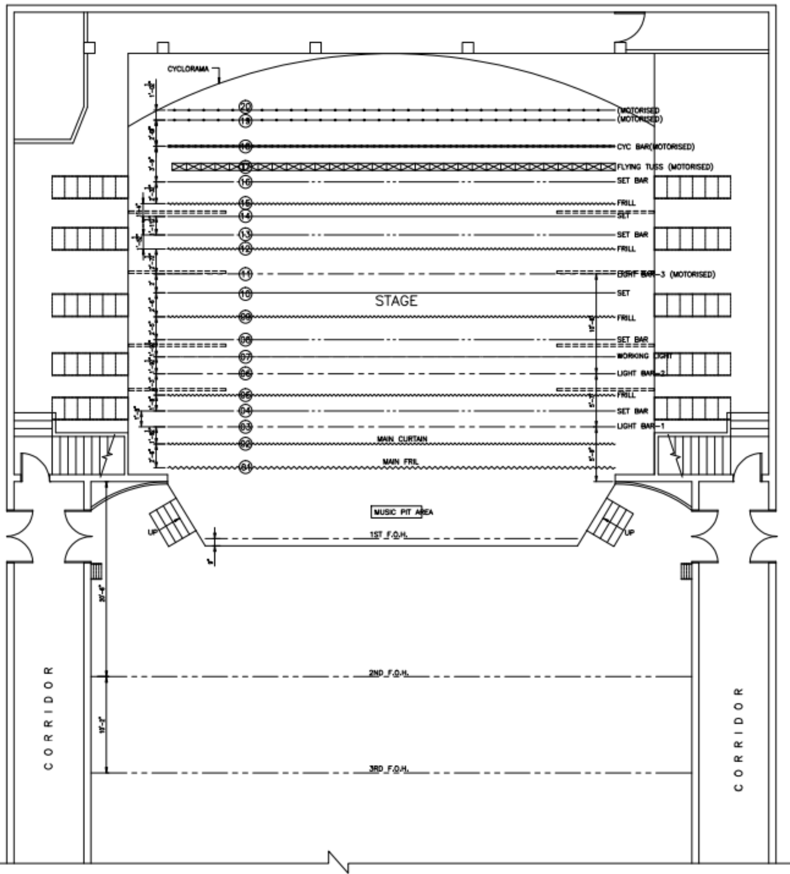
AUDITORIUM - STAGE BAR SYSTEM
