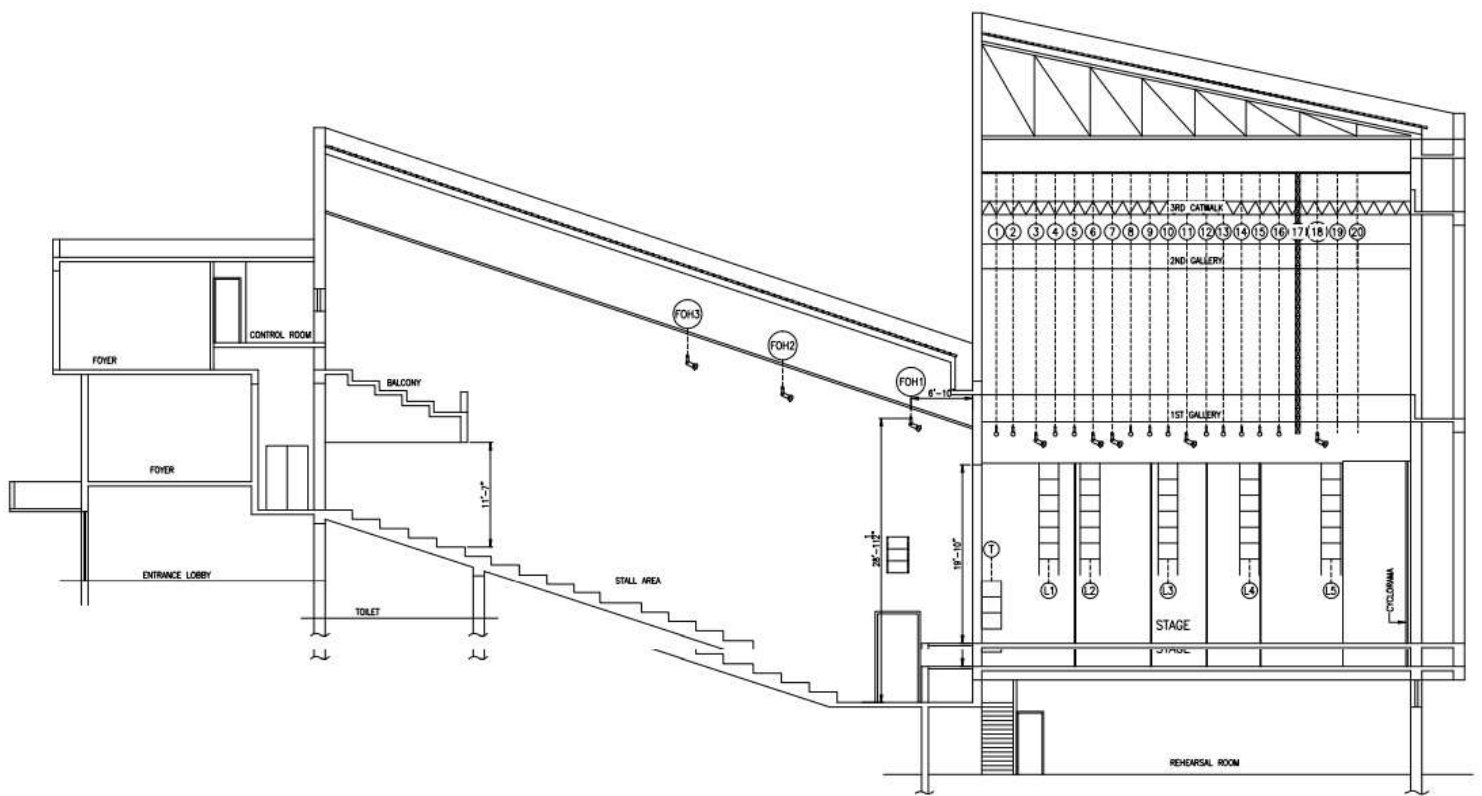
CROSS SECTION - AUDITORIUM
