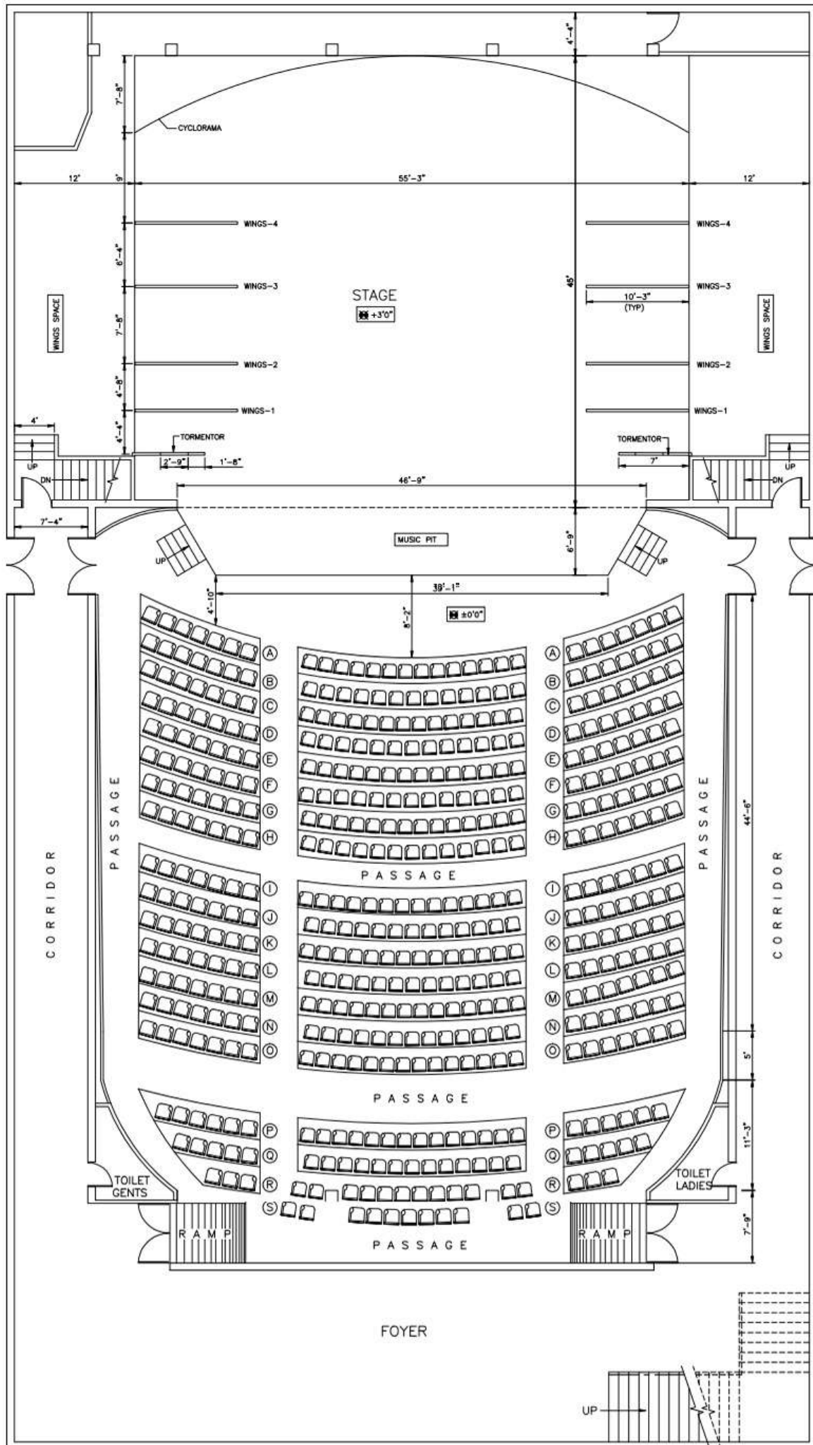
AUDITORIUM - GROUND PLAN
