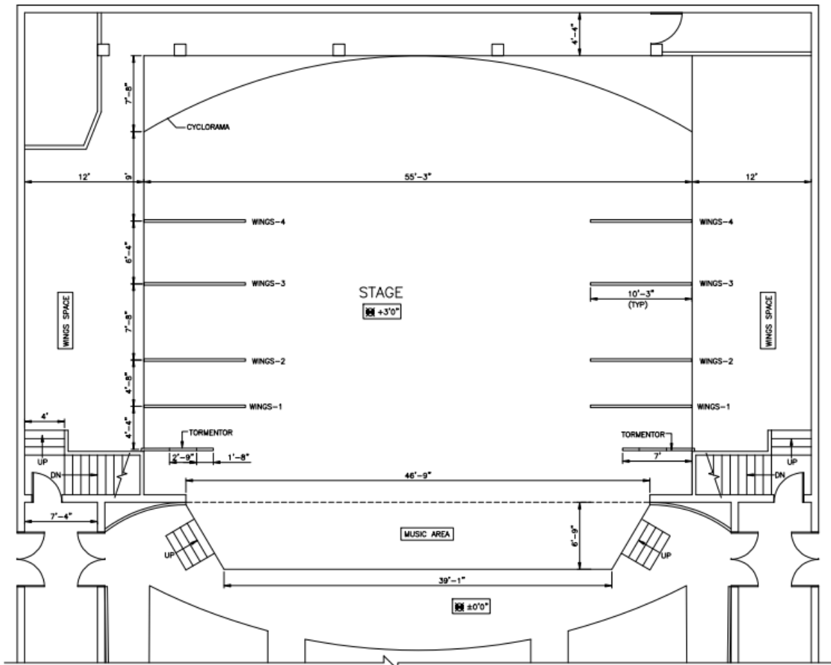
AUDITORIUM - STAGE PLAN
